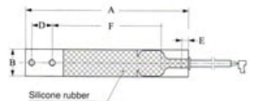
PW2D Single point
