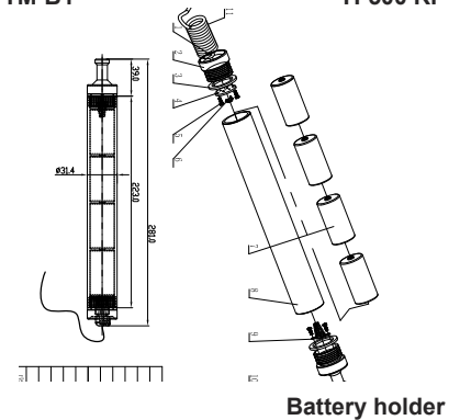
Battery holder
