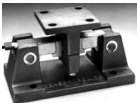
665016 w/ mounting assembly
