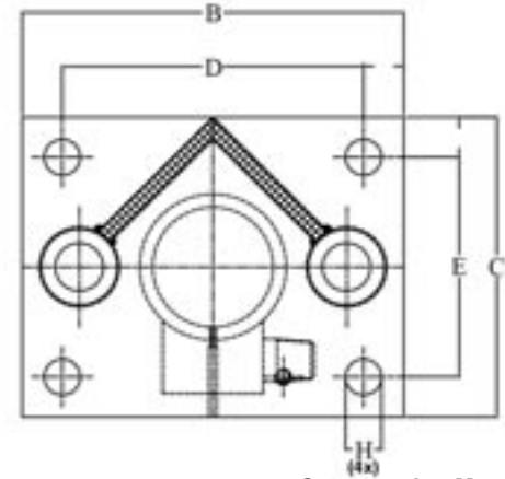
Compression Mount
