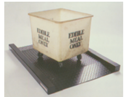
6950 Series Barrel Weighing Base built in ramps
