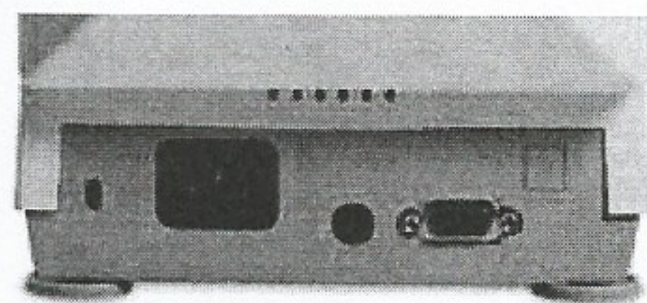
MB25/23 RS232 interface connection
