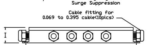
Fiberglass Enclosure
