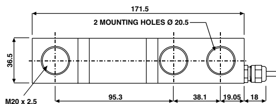
DIMENSIONS FOR CAPACITIES 3000 and 5000 kg
