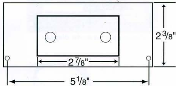
Panel Cutout for switch plate Allow 1 1/2" Clearance behind panel
