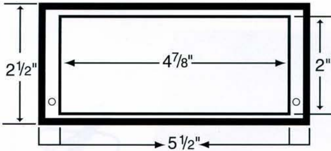
Panel Cutout for display Allow 1 1/2" Clearance behind panel
